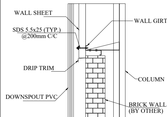
DRIP TRIM DETAIL
