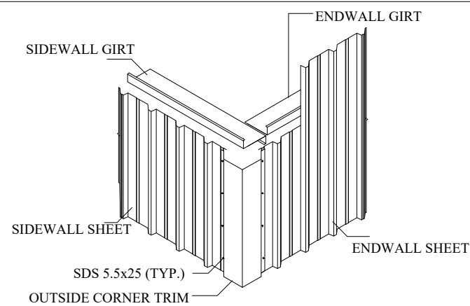
CORNER TRIM DETAIL (3-D)
